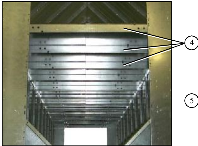
Plenum divider support channels.
